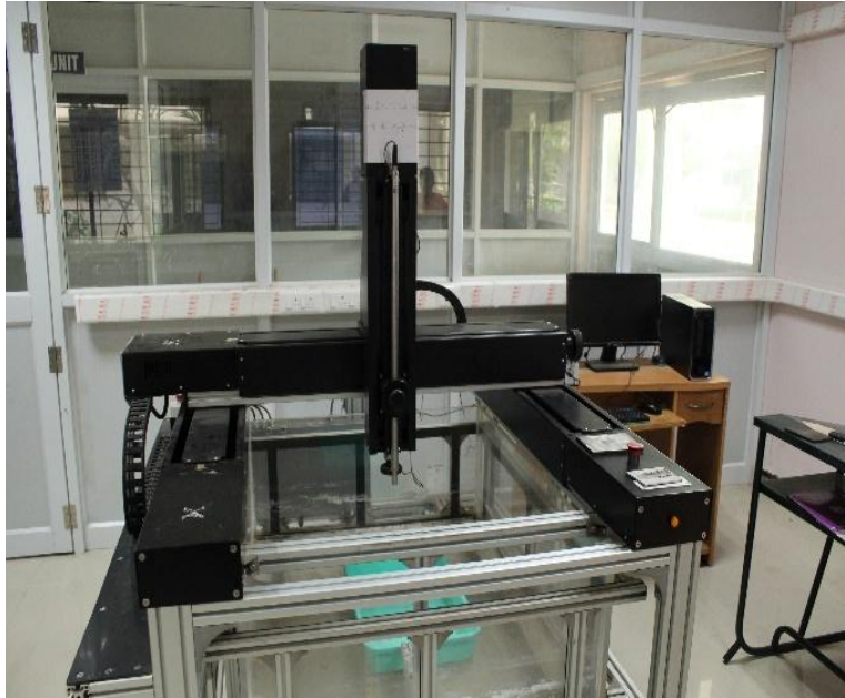
Ultrasonic C-Scan
